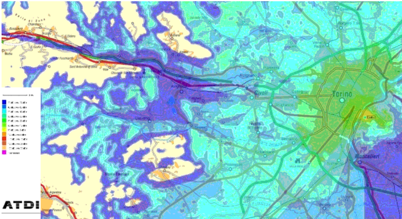
FIGURE 4 Coverage prediction
