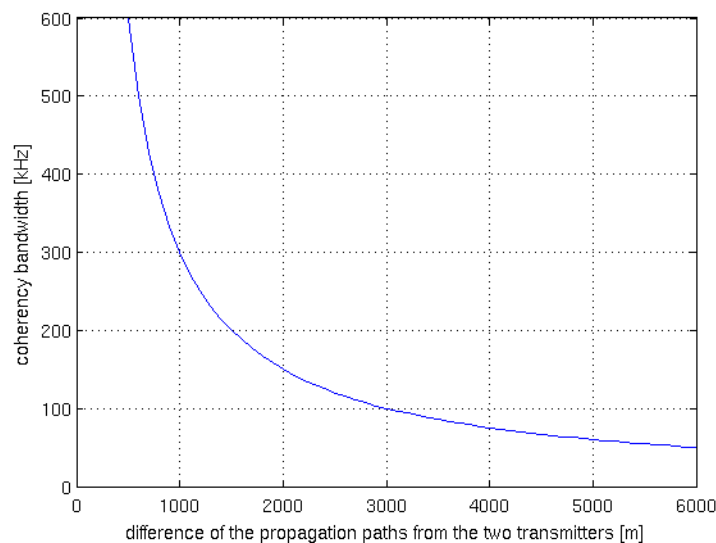
FIGURE 1 Coherence bandwidth in the overlapping area
