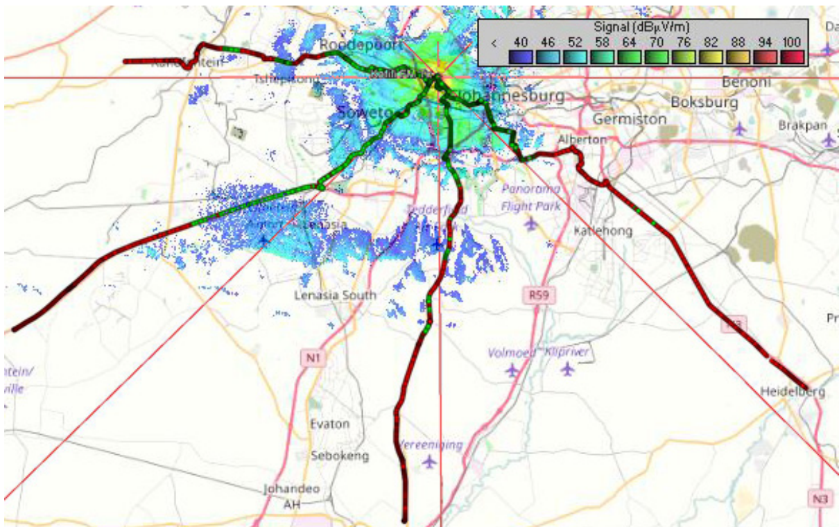
Drive-by mobile measurements at 16 QAM and 1/3 FEC against coverage prediction at 99% location probability and a threshold of 40 dBµV/m
