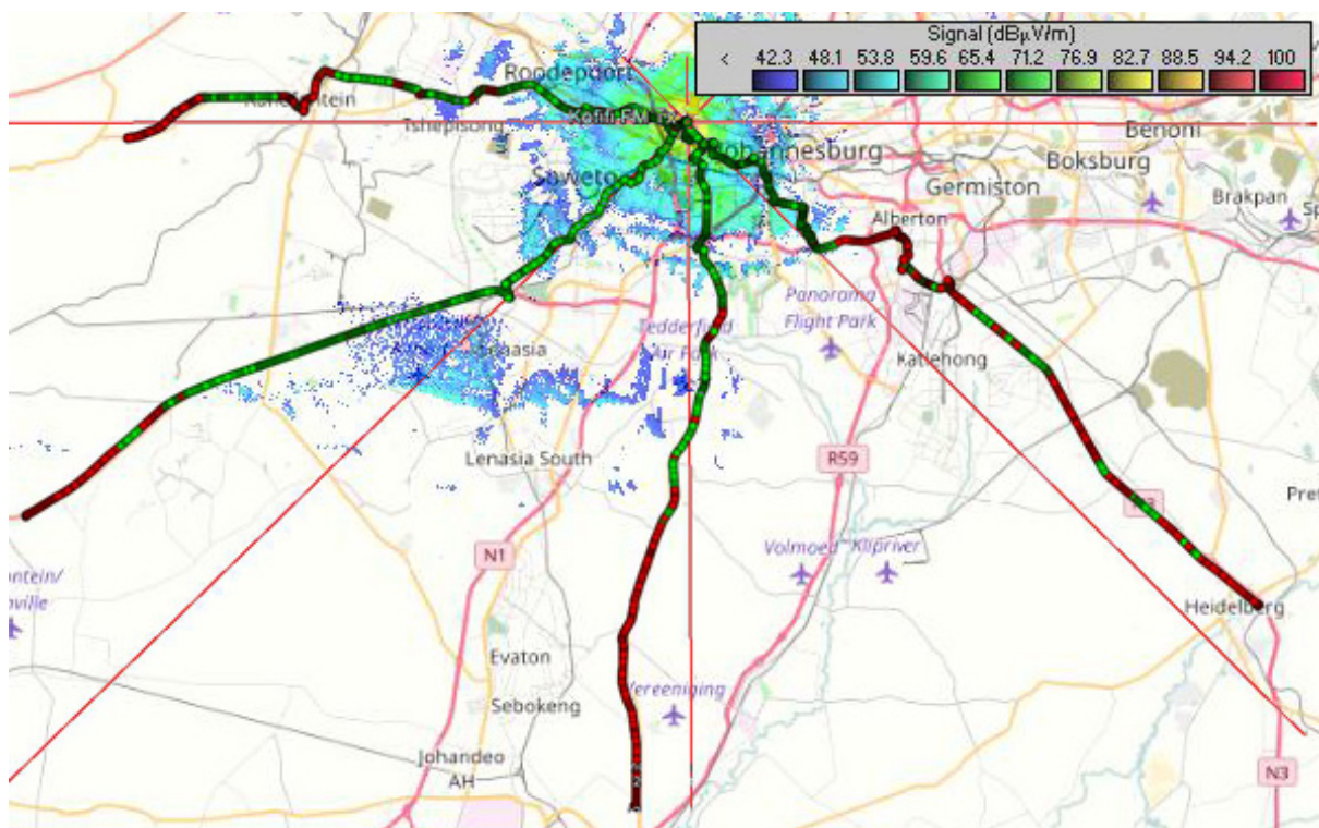
Drive-by mobile measurements at 4 QAM and 1/3 FEC against coverage prediction at 99% location probability and a threshold of 42.27 dB \mu V/m
