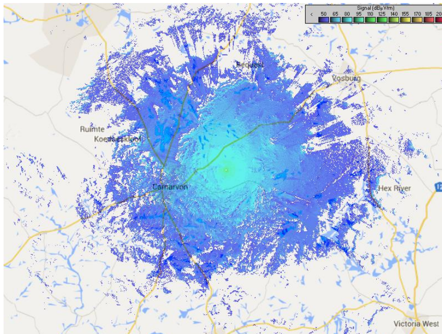
Predicted Coverage Map of the Karoo-DRM+ Multiplex
